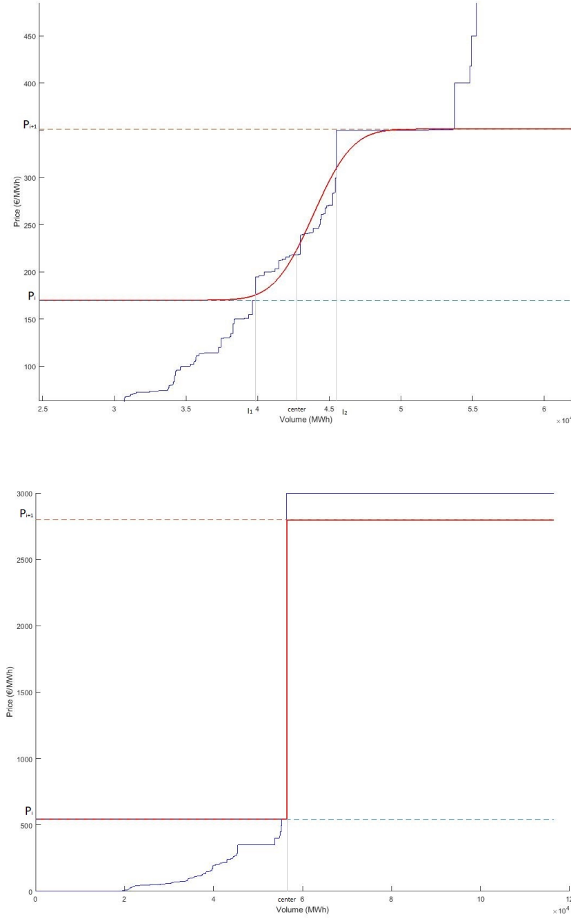
Figure 4.7: Local interpolation by one error function with lsqcurvefit function
